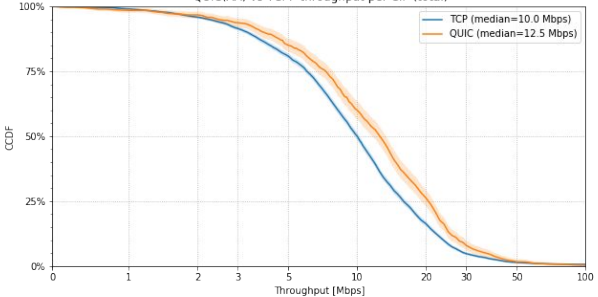
QUIC(AA) vs TCP: throughput per CIP (total)
